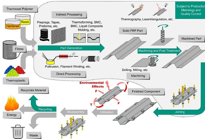
Figure 1: life cycle of FRP products (Fleischer et al., 2018)
